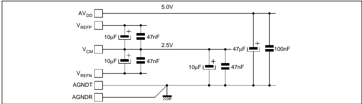
Figure 17 : Voltage Decoupling
