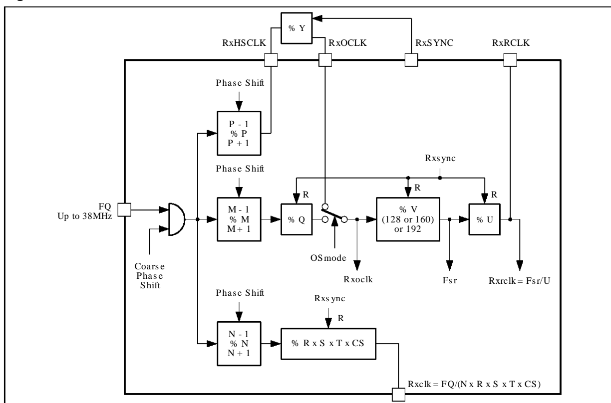
Figure 11 : Receive Clock Generator
