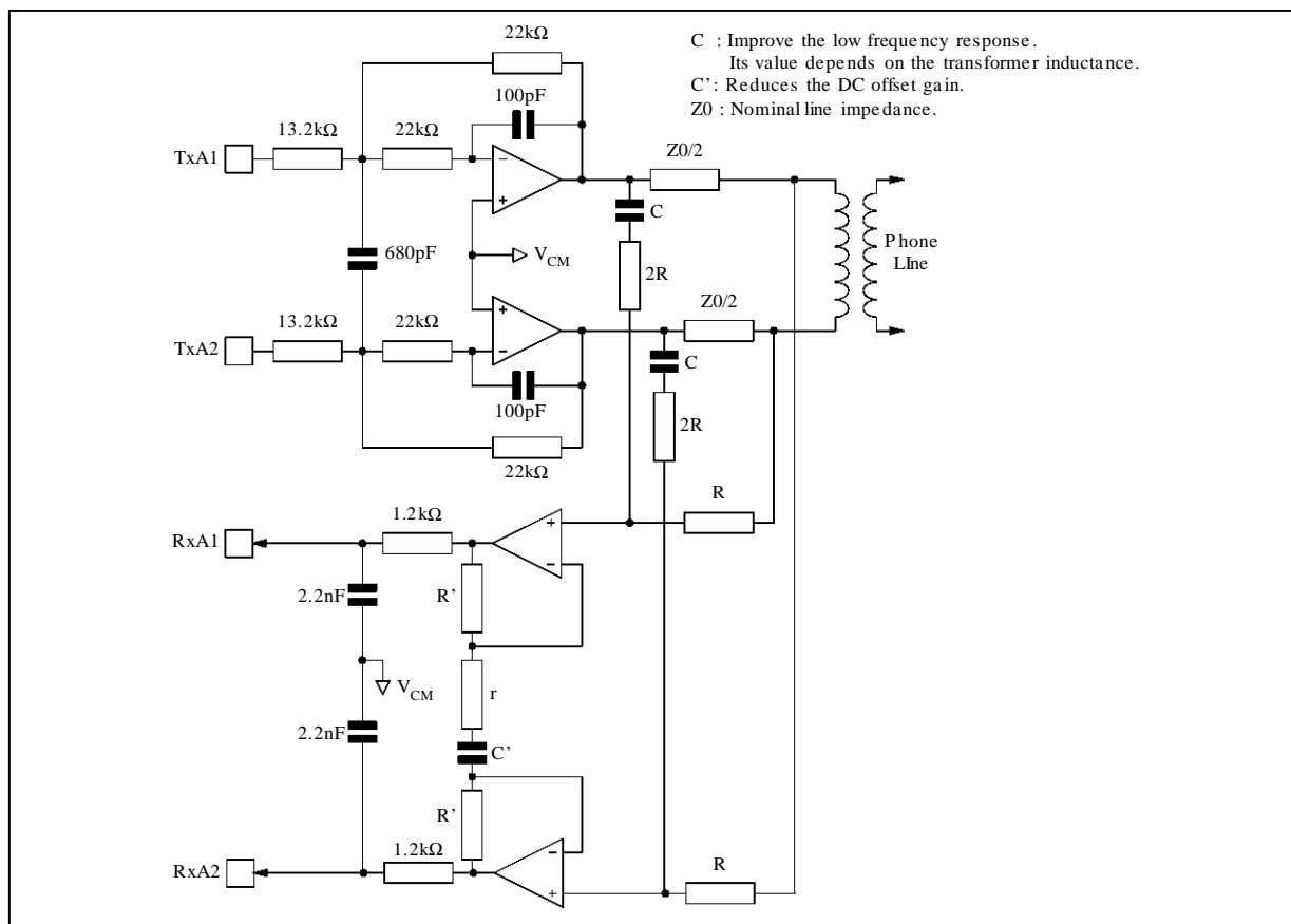
Figure 16 : Differential Duplexer
