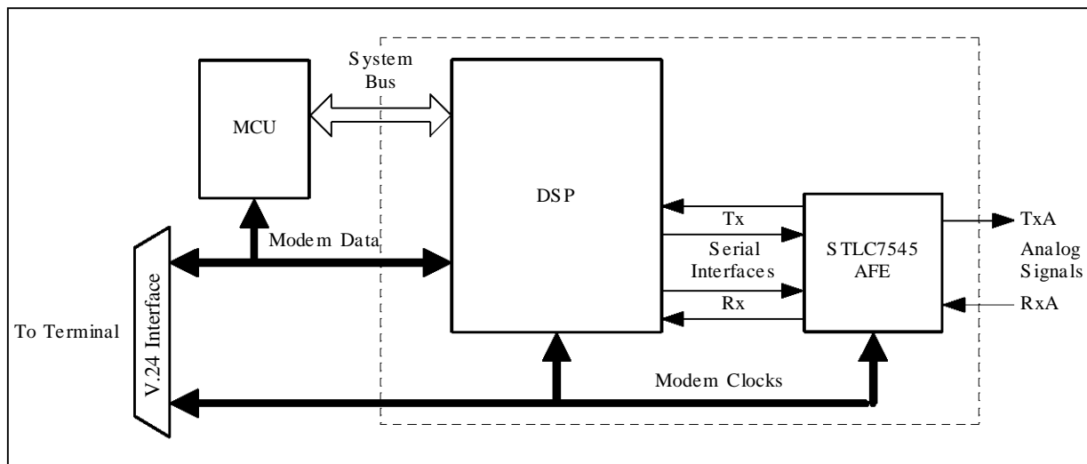
Figure 15 : Multistandard Modem with Echo Cancelling Capability
